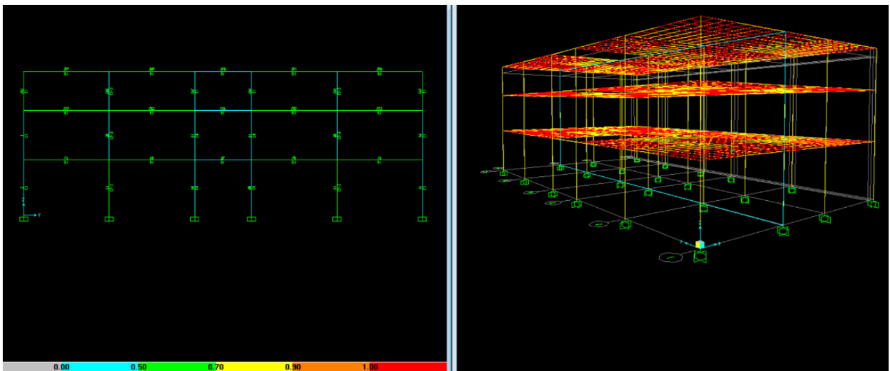
Figure 24. DCR of beams and columns after adding new story Internal frame; YZ-plane @ X=7.5m
