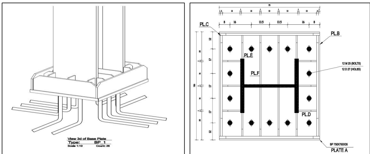
Figure 11. Column-Raft connection
