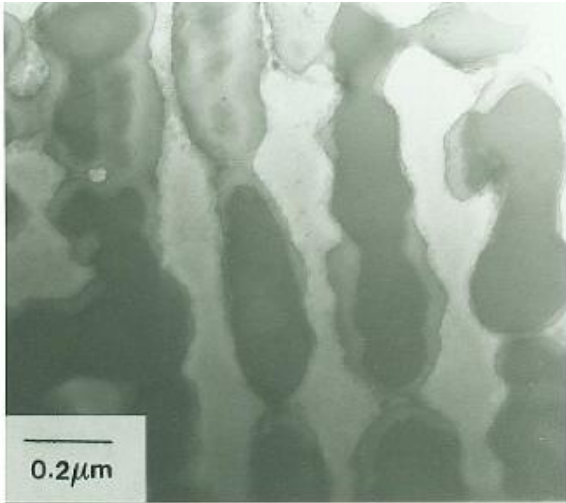
Figure 12 – Electron micrograph of Cu-45Ni-10Cr alloy during the later stages of ageing, showing more coarsened periodic structure (1 week aged at 800°C, \lambda \approx 3300\text{\AA} ) [19]
