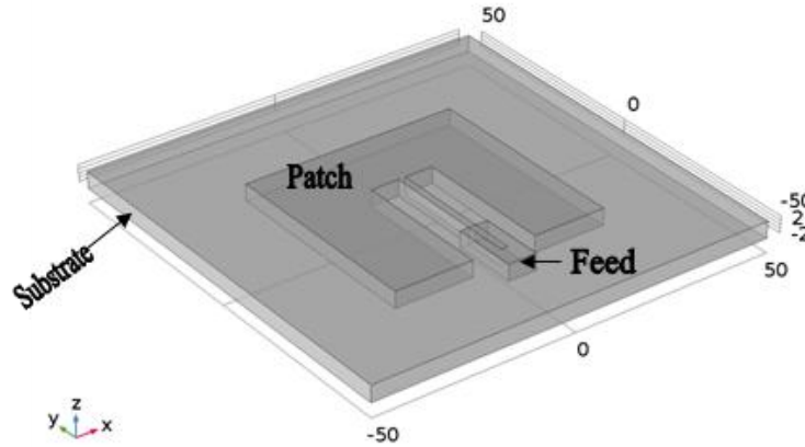
Figure 2. The proposed microstrip patch antenna
