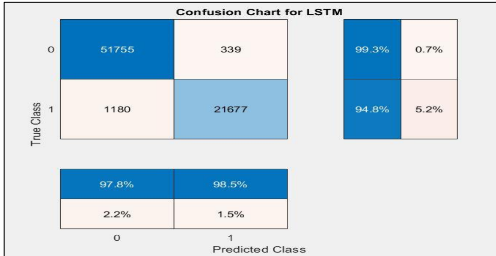
Figure 8. Confusion Chart for LSTM
