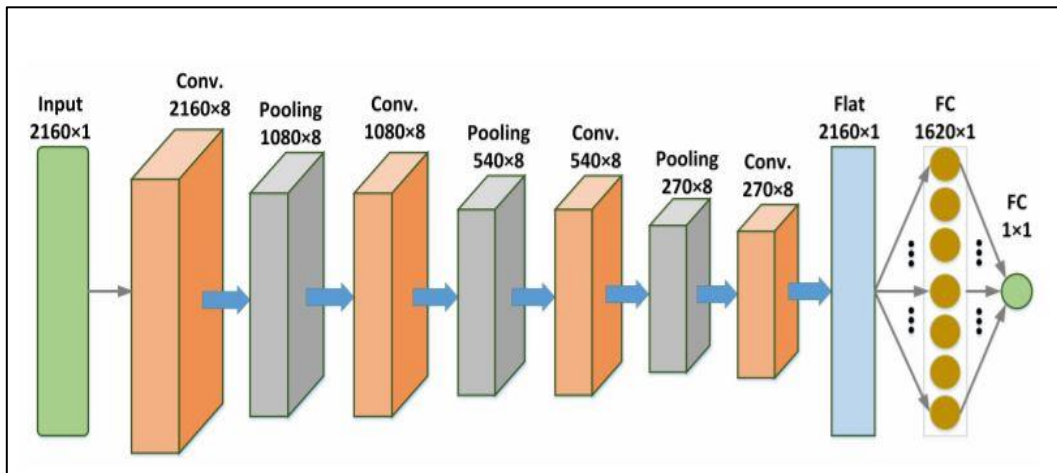
Figure 2. Proposed CNN architecture
