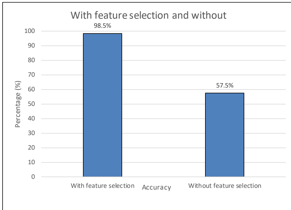
Figure 9. Results of experiment with and without feature selection
