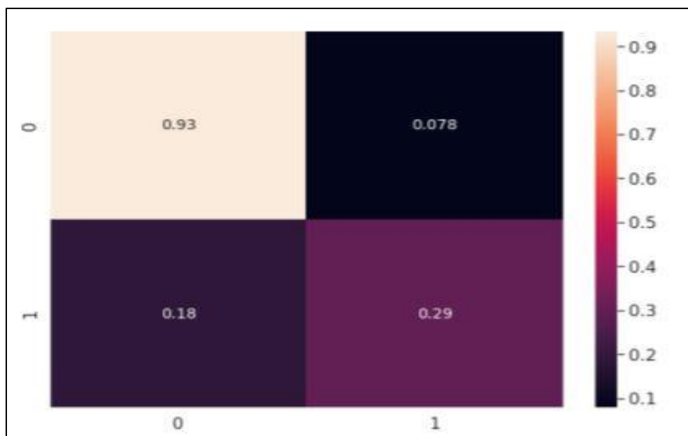
Figure 10. Confusion matrix
