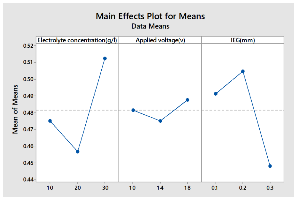
Figure 9. Influence of EC, V, and IEG on the removal rate
