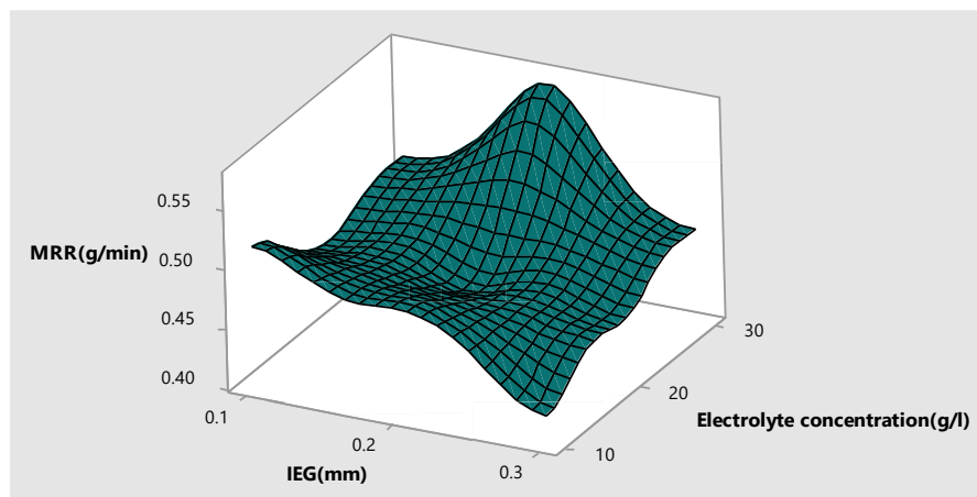
Figure 11. Relationship among material removal rate, inter electrode gap and electrolyte concentration.
