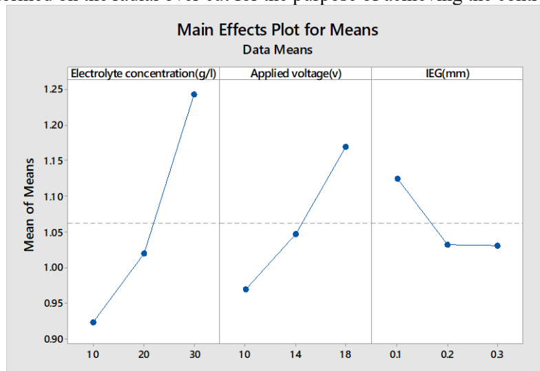
Figure 5. Influence of electrolyte concentration, voltage, and IEG on the ROC
