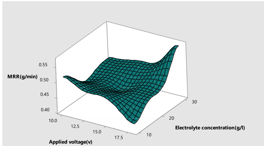
Figure 10. Relationship among material removal rate, Voltage and EC
