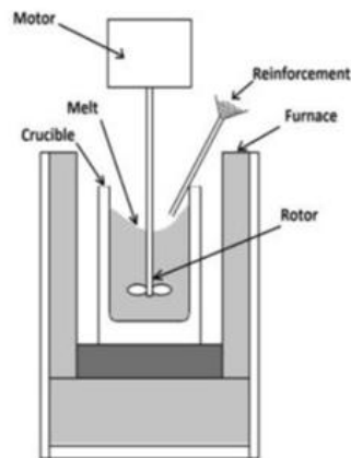
Figure 2. Stir casting principle
