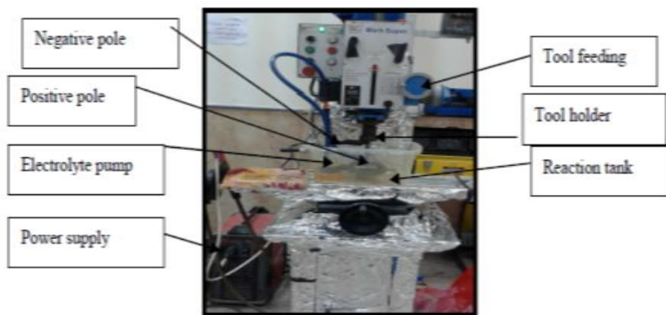
Figure 4. Electrochemical machining
