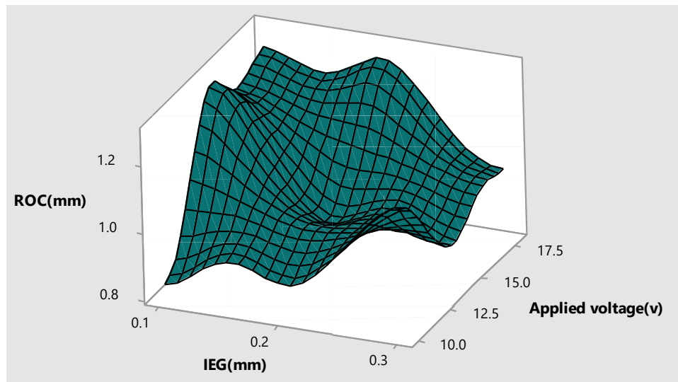
Figure 8. Relationship among radial over cut, inter electrode gap and voltage
