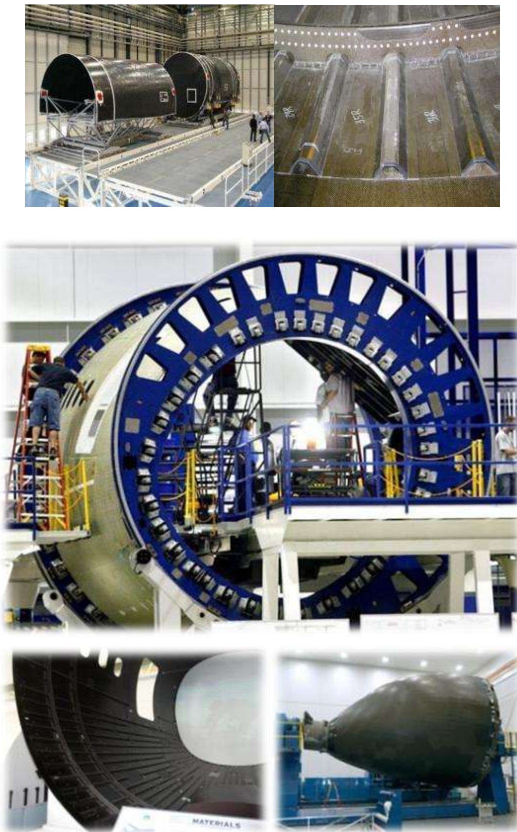
Figure 11 - Composite Material Usage in BOEING 787 Aircraft, Copyright of Boeing Commercial Airplanes, [12].
