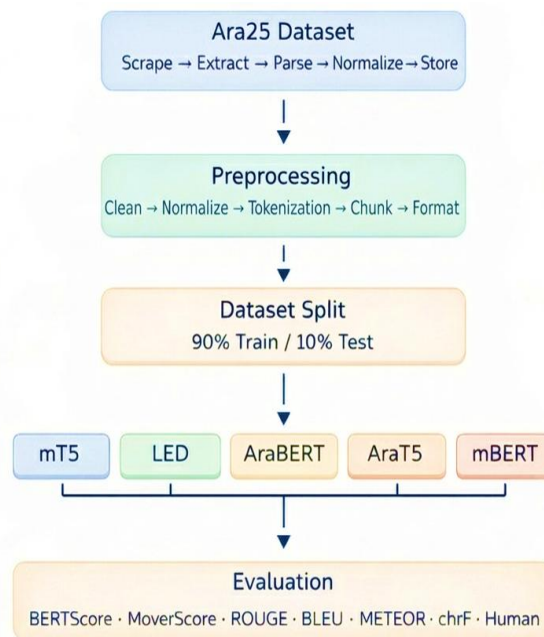
Figure 3. Schematic overview of the Ara25 training and evaluation pipeline
