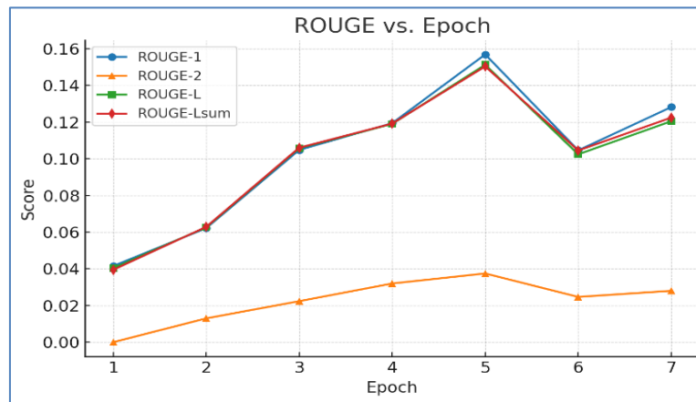
Figure 5. ROUGE curves viewing optimization across epochs
