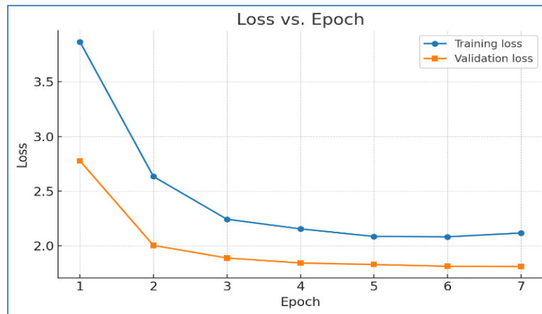
Figure 4. Loss curves showing optimization stability and convergence speed across epochs under the final training configuration
