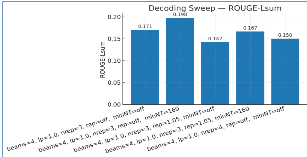
Figure 6. ROUGE-Lsum scores across different decoding configurations
