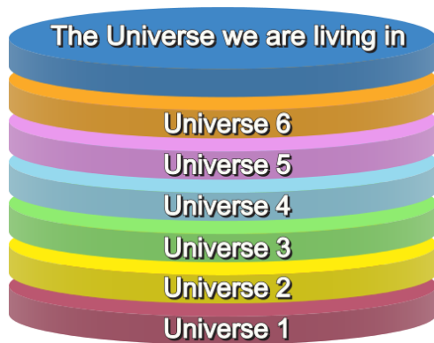
Figure 4: "Bubble universes": every disk is a bubble universe (Universe 1 to Universe 6 are different bubbles; they have physical constants that are different from our universe); our universe is just one of the bubbles. [20]
