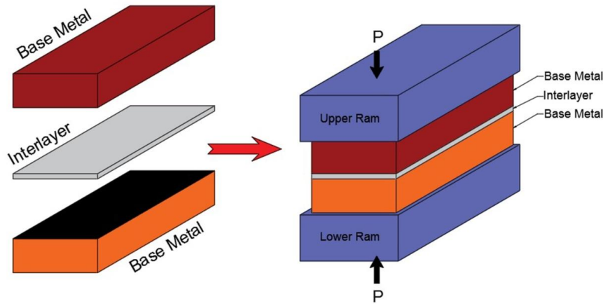
Figure 1: Processing system of diffusion welding
