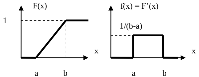
Figure 1. Uniform CDF and PDF
