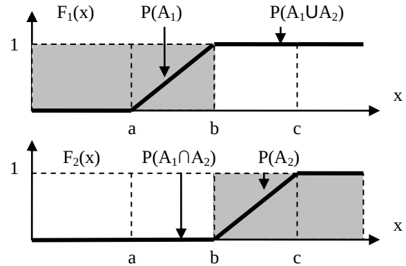
Figures 4. Method 1: CDF's F_1(x) and F_2(x)
