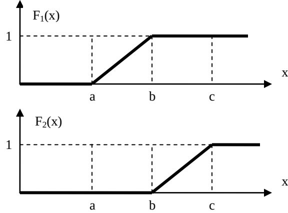
Figures 3. CDF's F_1(x) and F_2(x)
