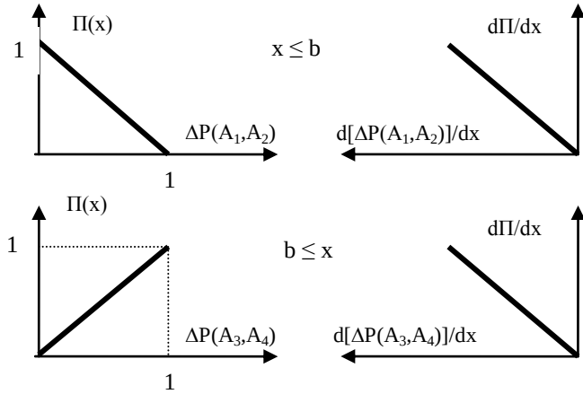
Figures 12: Method 2: Theorem 3 and Corollary 3
