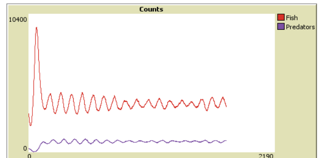
Figure 19. Unstable system predator parameters
