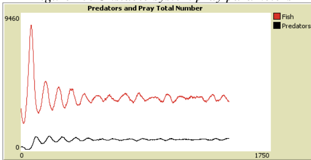
Figure 14. Unstable predator-prey system
