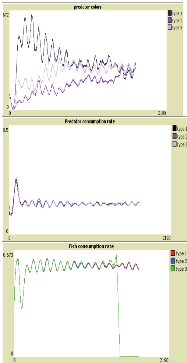
Figures 20. Results for Example 2 unstable system
