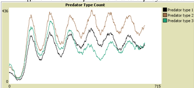
Figure 5. Detailed three predators count
