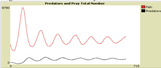
Figure 4. Total 3 predators and 3 preys count
