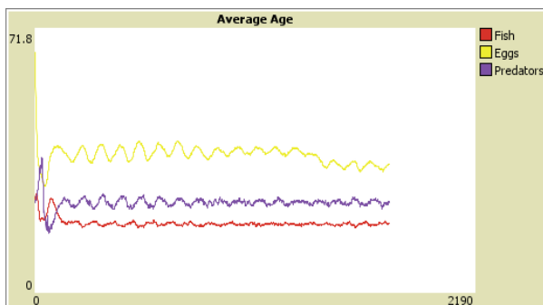
Figures 21. Example 2 average age, preys, predators
