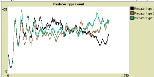
Figure 16. Unstable system detailed count of predators
