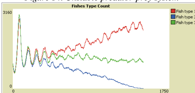
Figure 15. Unstable system detailed count of preys
