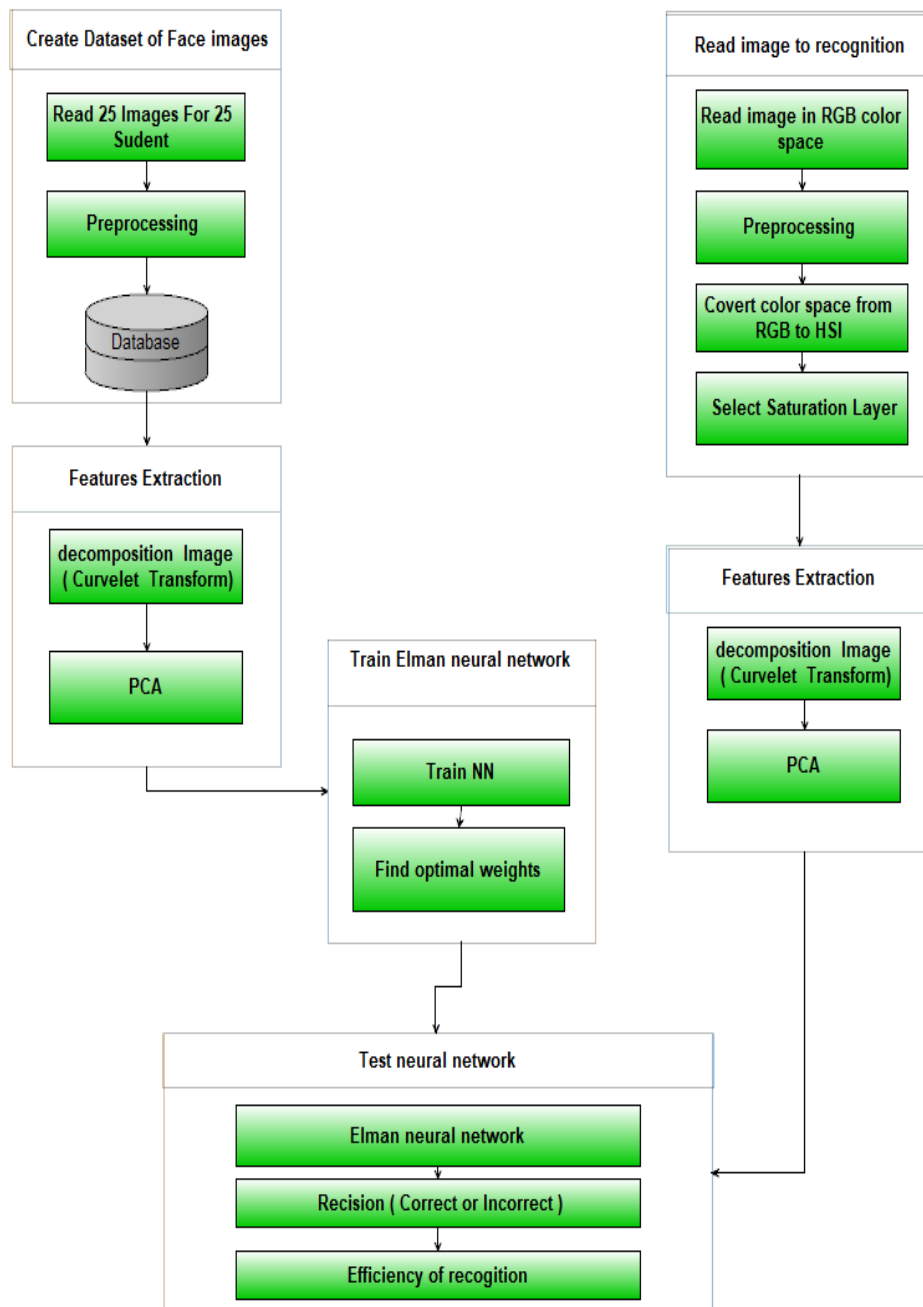
Figure 3. Proposed algorithm
