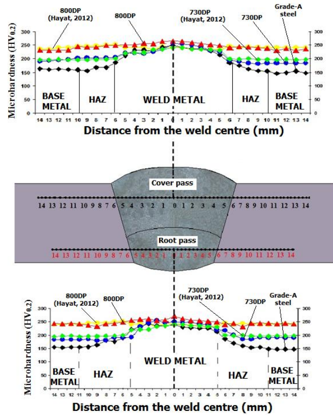
Figure 6. Hardness profiles along the top and bottom in cross-section of the Grade-A and dual phase steels
