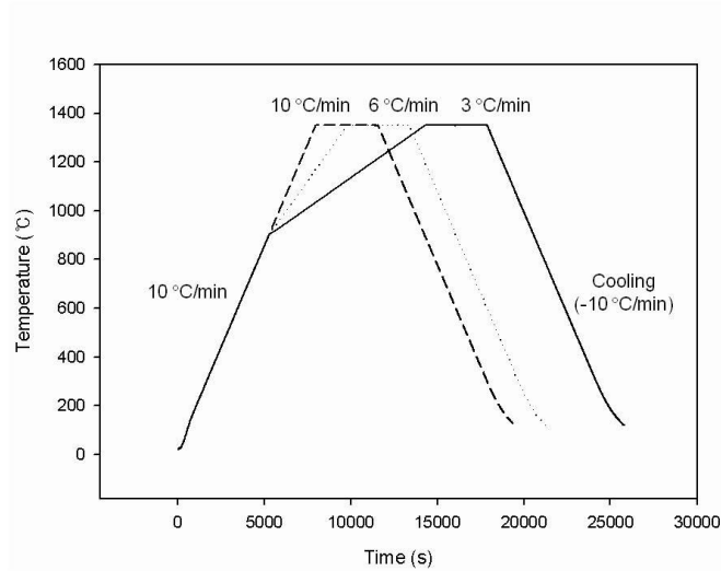
Figure 3. Thermal history of dilatometry experiments.
