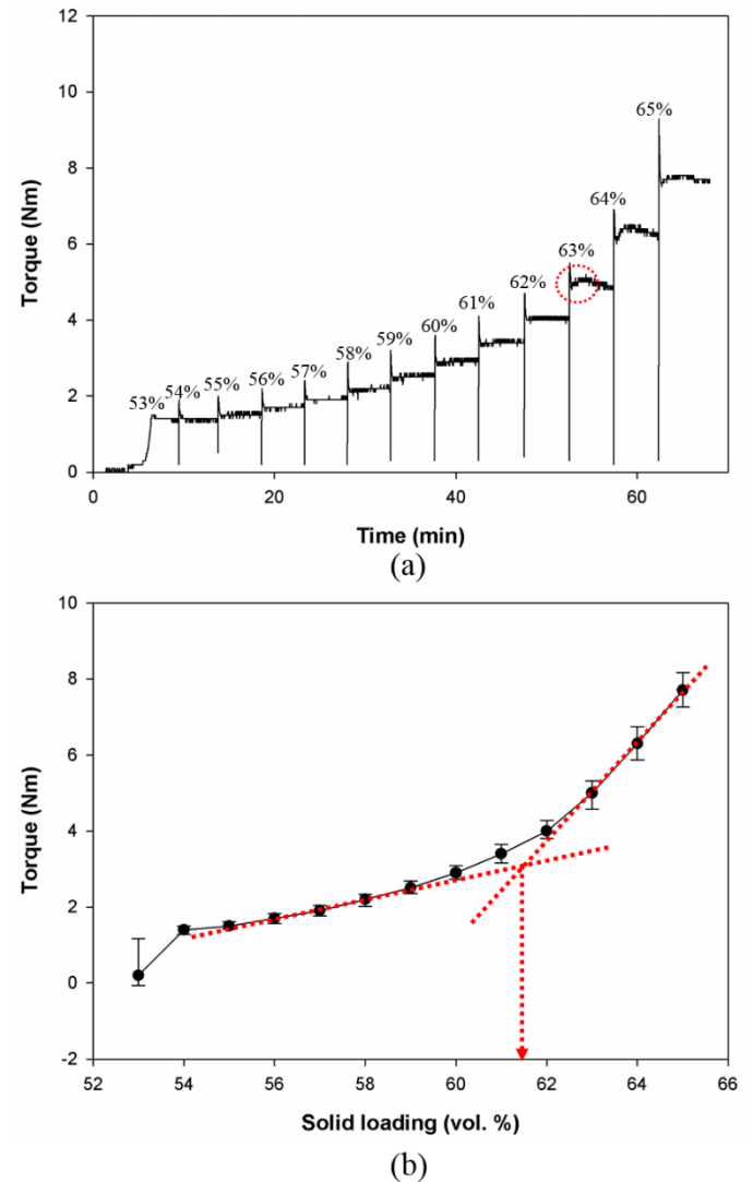
Figure 4. Mixing torque, (a) as a function of time, and (b) as a function of solid loading.
