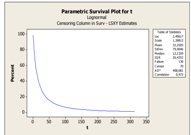
Figure 4. Parametric Lognormal Survival Function
