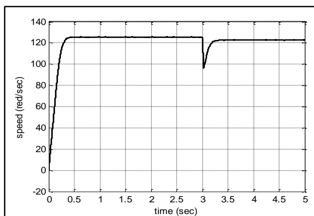
Figure 9. Motor speed response with PI controller ( f=40 Hz) with sudden load TL = 5 Nm at t = 3 sec.
