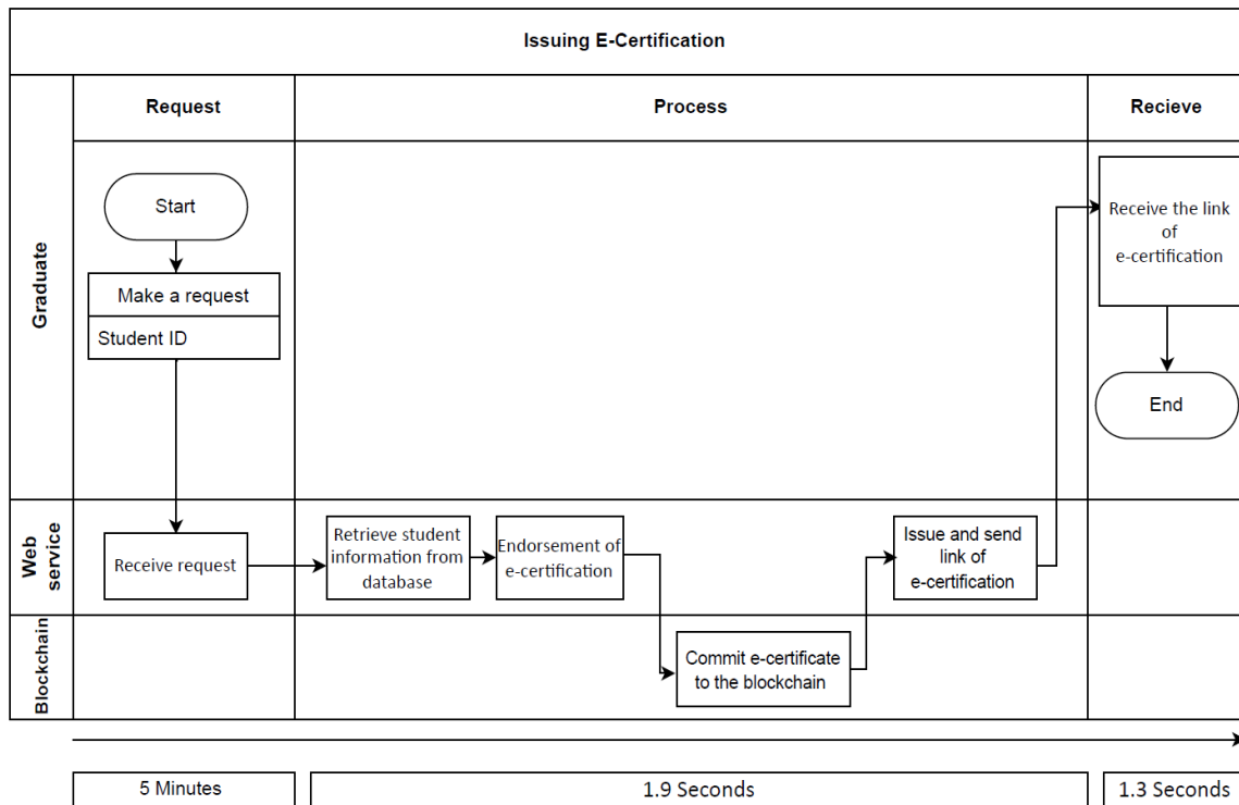
Figure 4. Issuing e-certificate process
