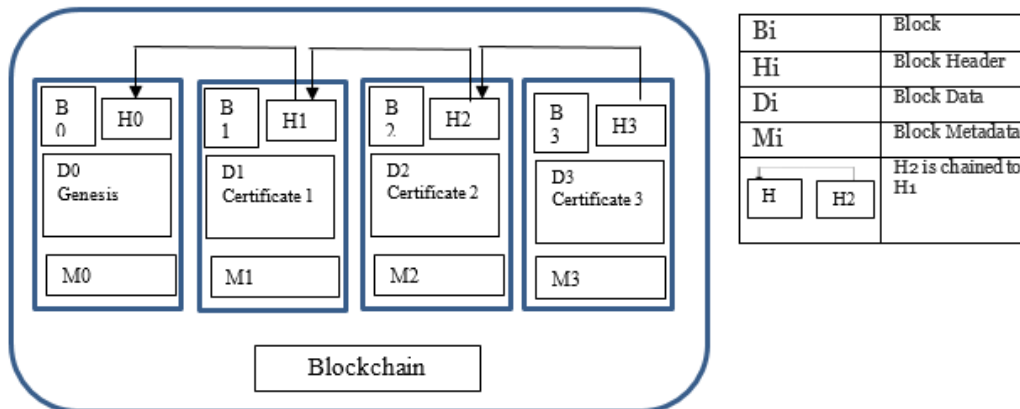
Figure 7. The blockchain components of the proposed system
