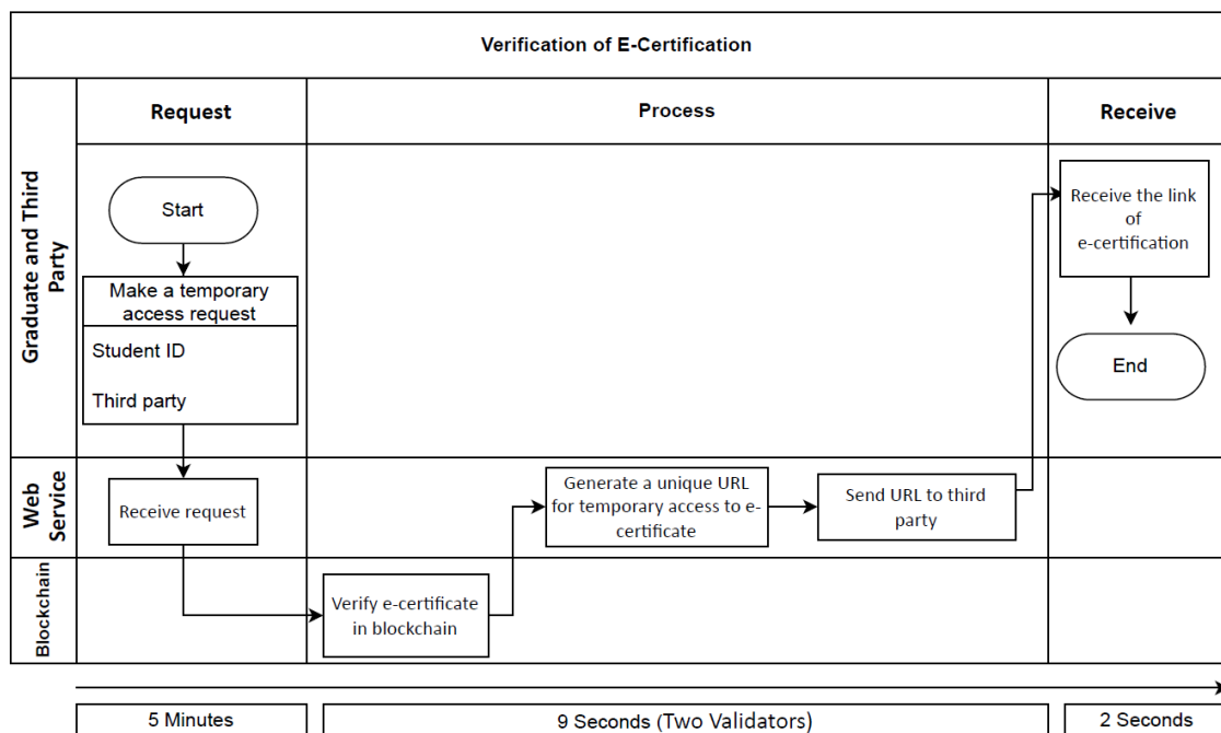
Figure 5. Certification verification service
