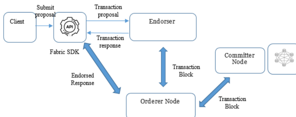
Figure 1. Hyper ledger Fabric components
