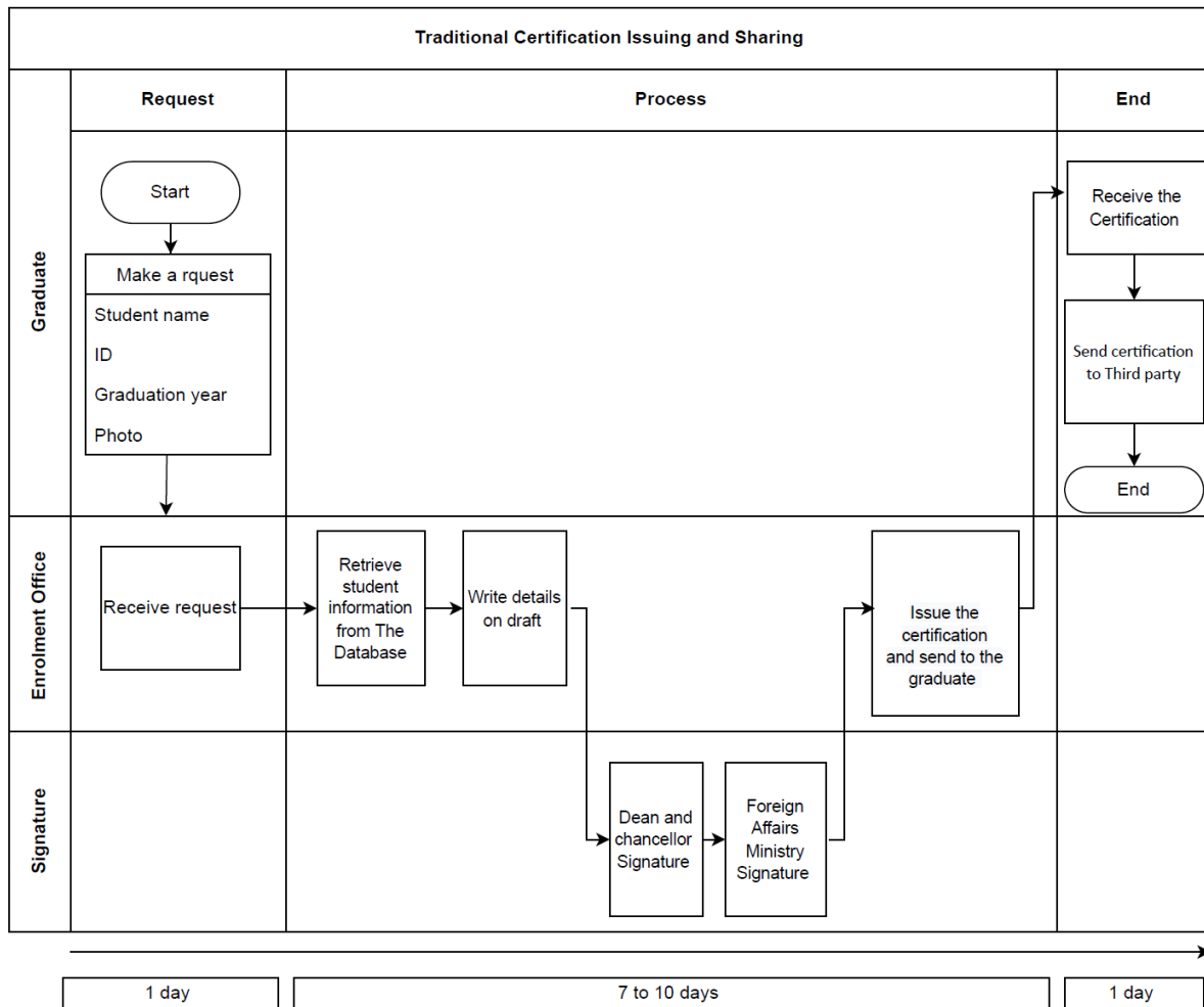
Figure 3. The timeline to issue a graduate certification at UoT -Iraq
