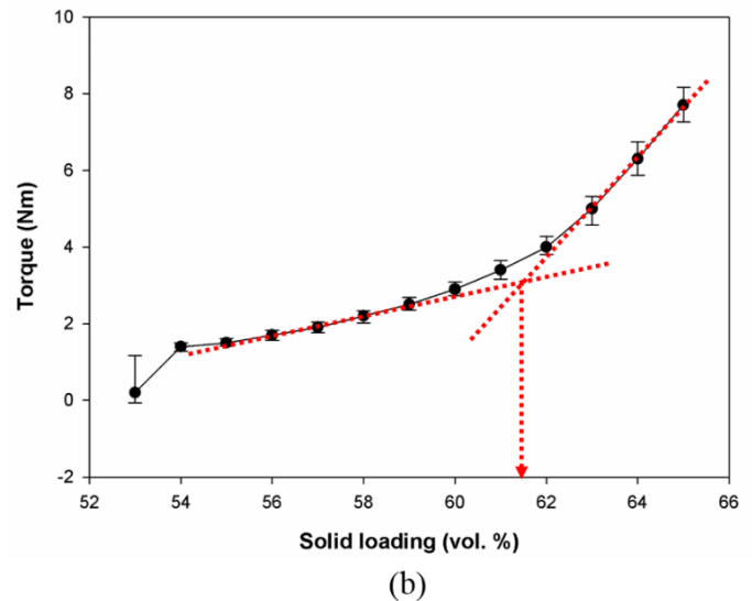
Figure 4. Mixing torque, (a) as a function of time, and (b) as a function of solid loading.
