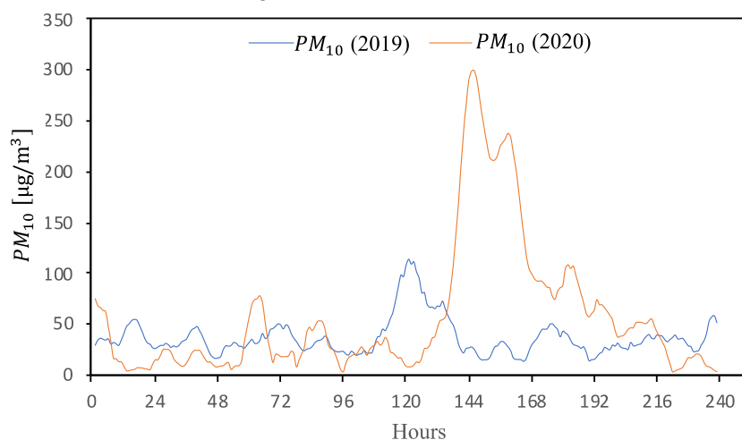
Fig. 4. Concentration of PM_{10} for the second phase in March 2019 and March 2020
