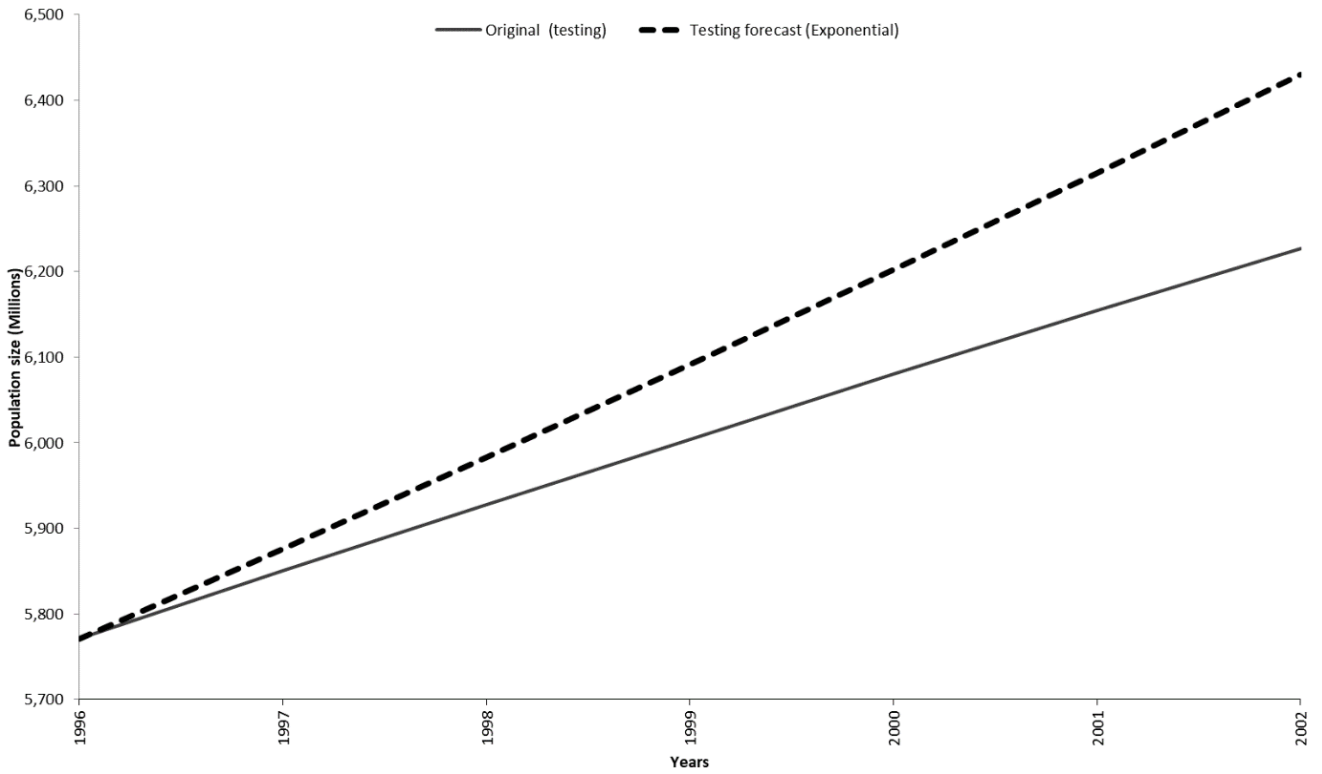
Figure 6. The fitness of original testing series using exponential method
