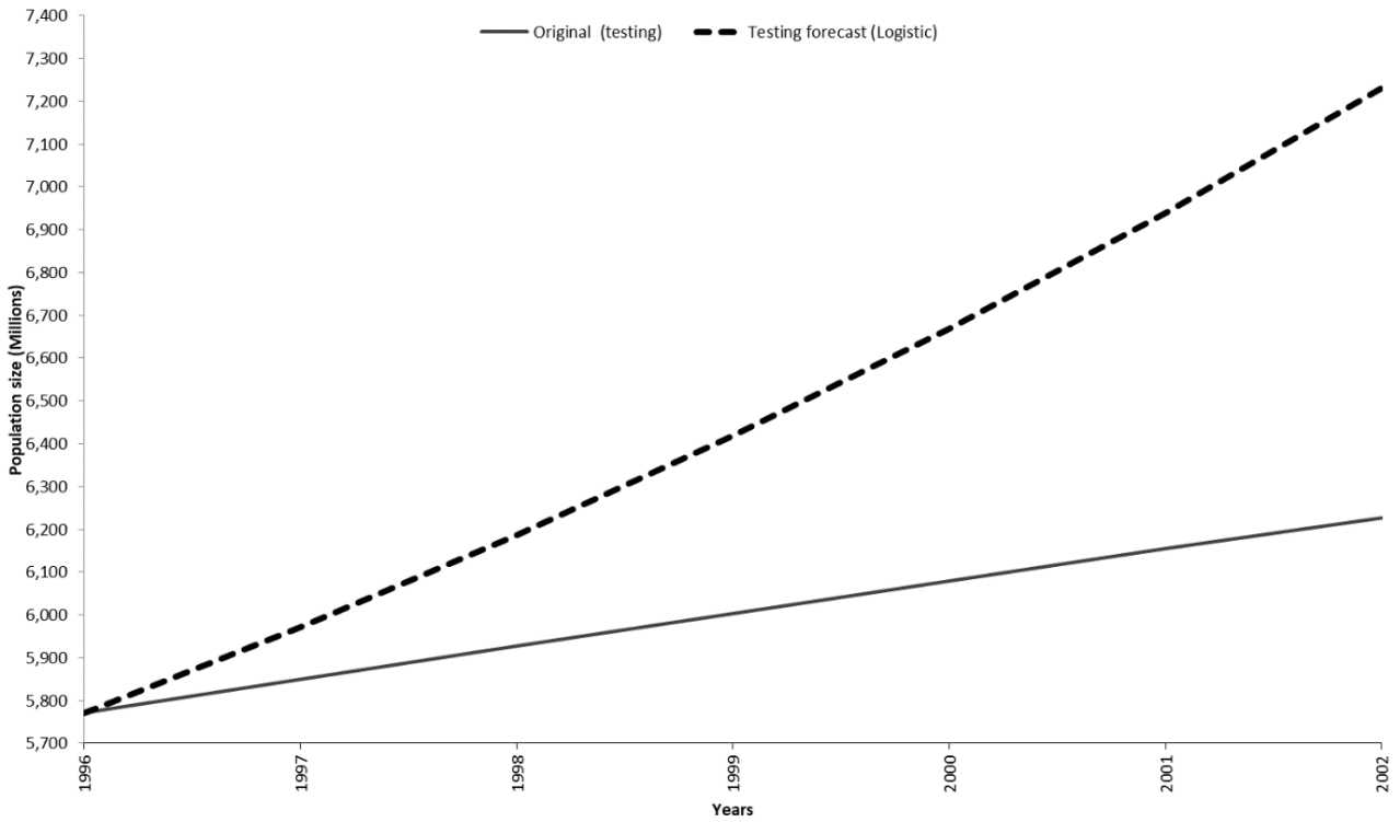
Figure 8. The fitness of original testing series using logistic method
