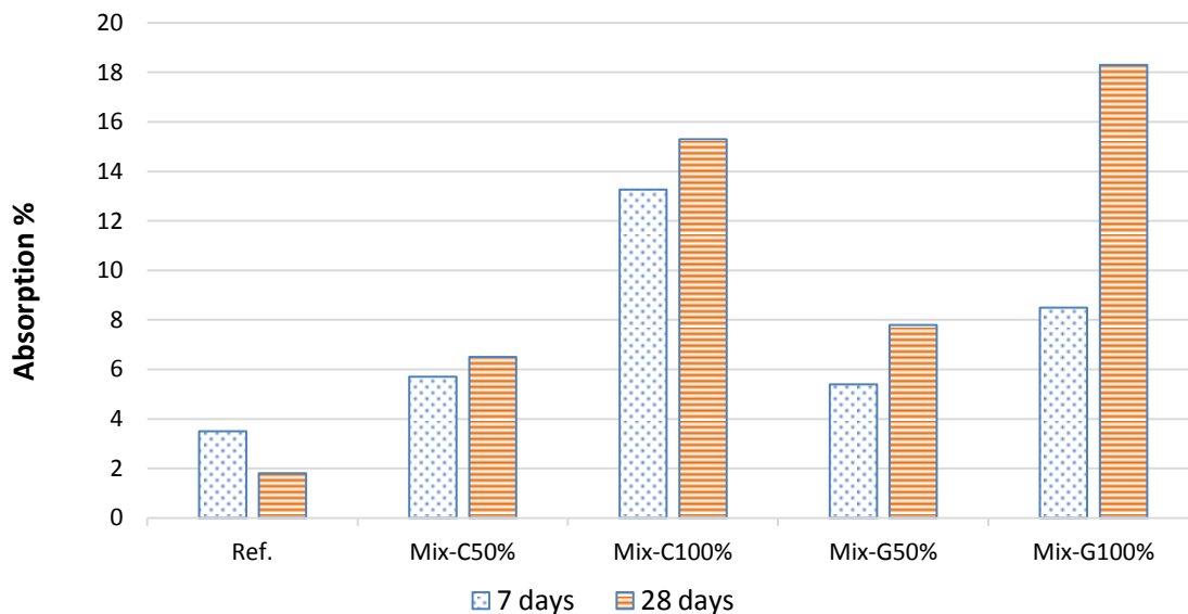
Figure 6. Total absorption for all mixes
